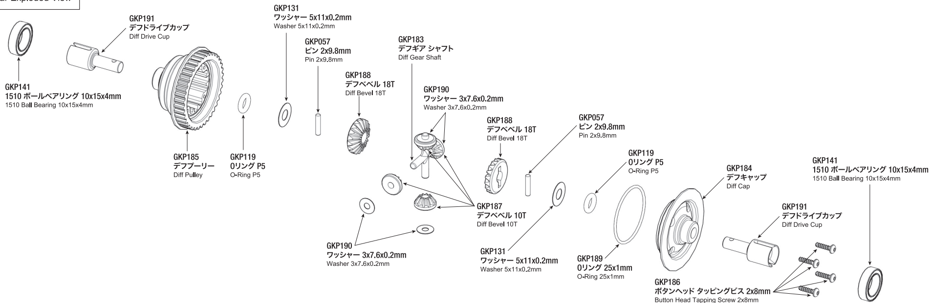
デフギア展開図 Diff Gear Exploded View
